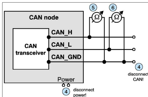
Figure 12: Measuring the internal resistance of CAN transceivers
