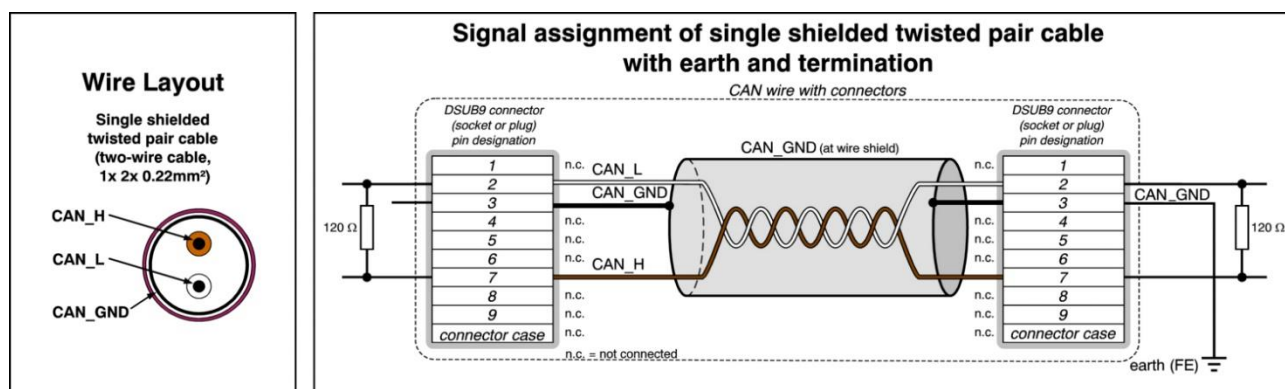
Figure 6: CAN wiring for light industrial environment
